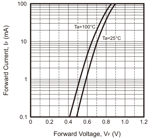
Fig.1 - Forward Characteristics (CDSV3-202N-HF)
