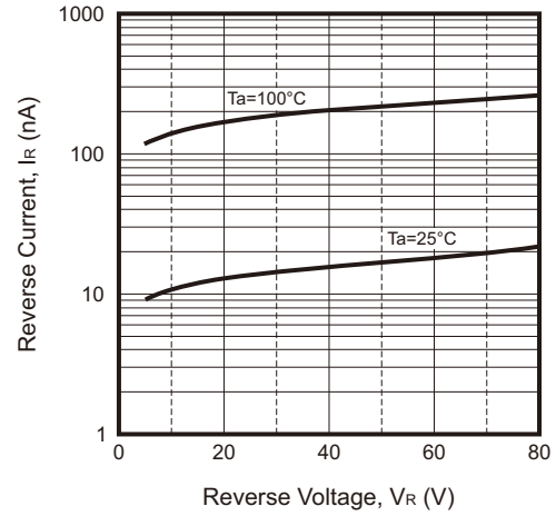
Fig.2 - Reverse Characteristics (CDSV3-202N-HF)
