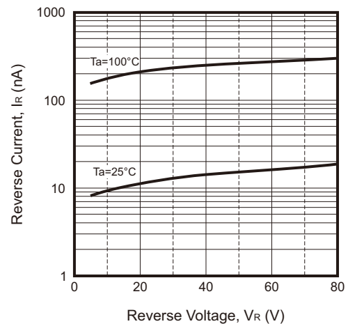
Fig.4 - Reverse Characteristics (CDSV3-202P-HF)
