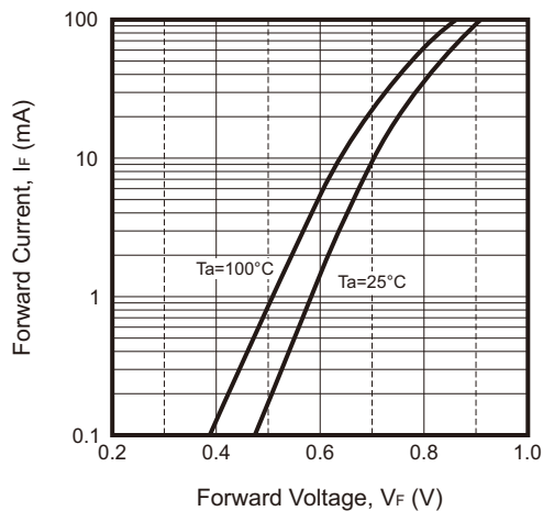
Fig.3 - Forward Characteristics (CDSV3-202P-HF)
